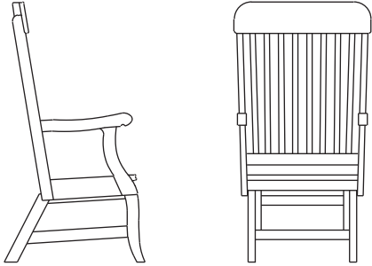
ROC01 Stable Base Rocker 28"d x 26"w x 45"h 27" arm ht 17" seat ht 35" rocking depth, 28" stable depth
