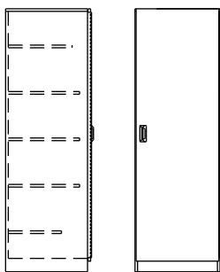
PSA01S3 Wardrobe, One-Door w/ Three Shelves 24"d x 24"w x 74"h
