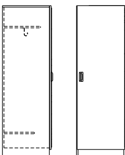
PSA01S Wardrobe, One-Door 24"d x 24"w x 74"h
