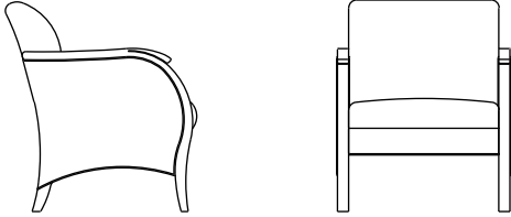
SF601 Orsay Chair 28.5"d x 24.5"w x 31.5"h 26" arm ht 19.5" seat ht
