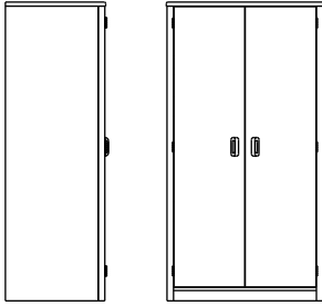
GC01S Wardrobe w/2 Doors & Shelf 24.25"d x 37.75"w x 72.25"h
