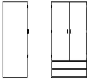
RC02 Wardrobe, 2-Door & 2 Drawers 24"d x 36"w x 74.75"h
