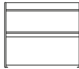
RM09DT36 10"d x 42"w x 32.75"h (also RM09DT36N - 36"w RM09DT36W - 48"w)
