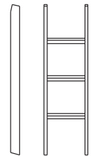
RM72 3"d x 14.5"w x 48.5"h (also RM72LG2 - 60.5"h)
