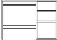
RM05 24"d x 42"w x 29.5"h (also RM05W - 48"w)
