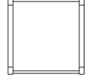
PASFT Public Area Seating Free Standing Table 23"d x 23"w x 16"h
